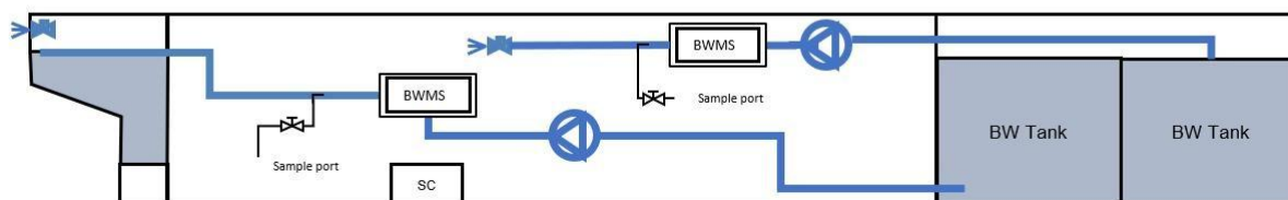
During discharge, sequential sampling can be performed from each dedicated tank resulting in two or more samples representing the respective BWMS
