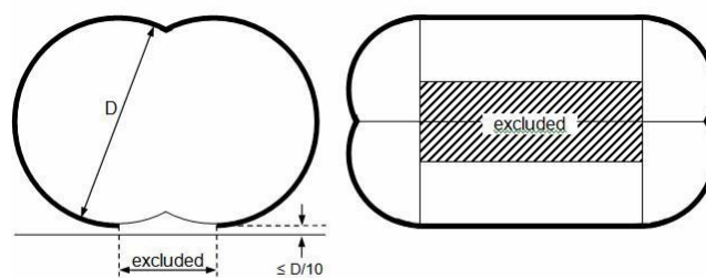
Bilobe tanks
