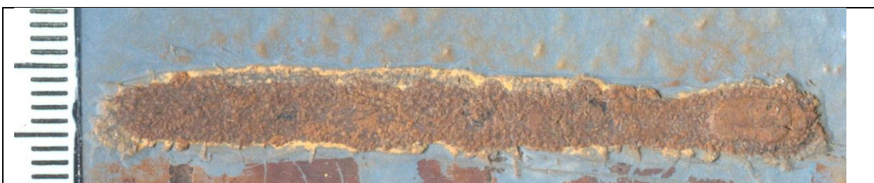
Figure C-5 Undercutting from scribe, side wave tank panel without cooling (example picture not connected to example results in this model report).
