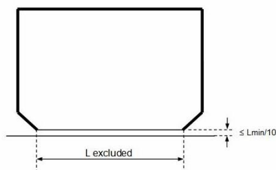
Prismatic tanks
