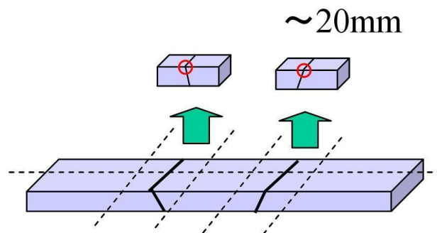
Figure App 3 - Sectioning plan
