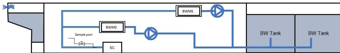
Ballasting utilising several BWMS in parallel and by mixing the treated water into ballast tanks.
