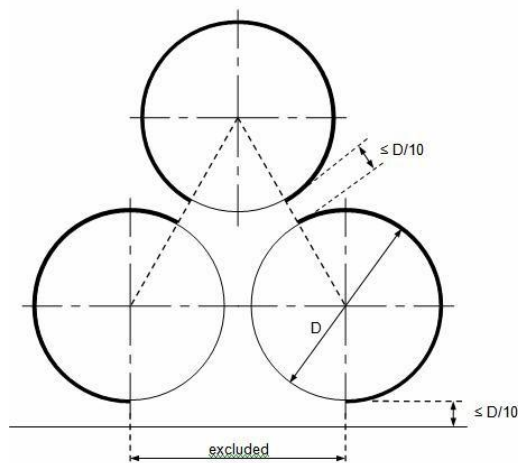
Horizontal cylindrical tanks arrangement
