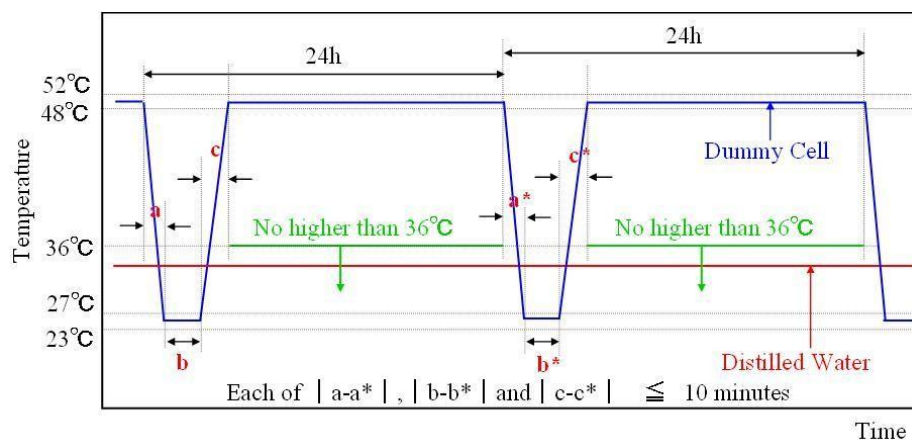
Figure App 1 - Schematic view of temperature controlling accuracy of specimens and distilled water during corrosion test
