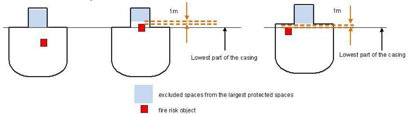
Figure 1 Machinery space including a casing
