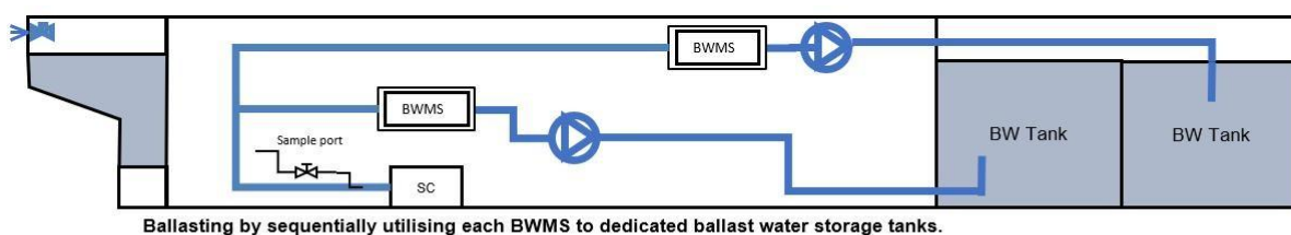
Ballasting by sequentially utilising each BWMS to dedicated ballast water storage tanks.
