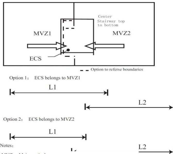
Figure 2: ECS serves two MVZ
