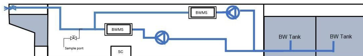
During discharge, sampling can be performed from one sample point located at a common overboard line, resulting in one sample representing treated water from all the respective BWMS
