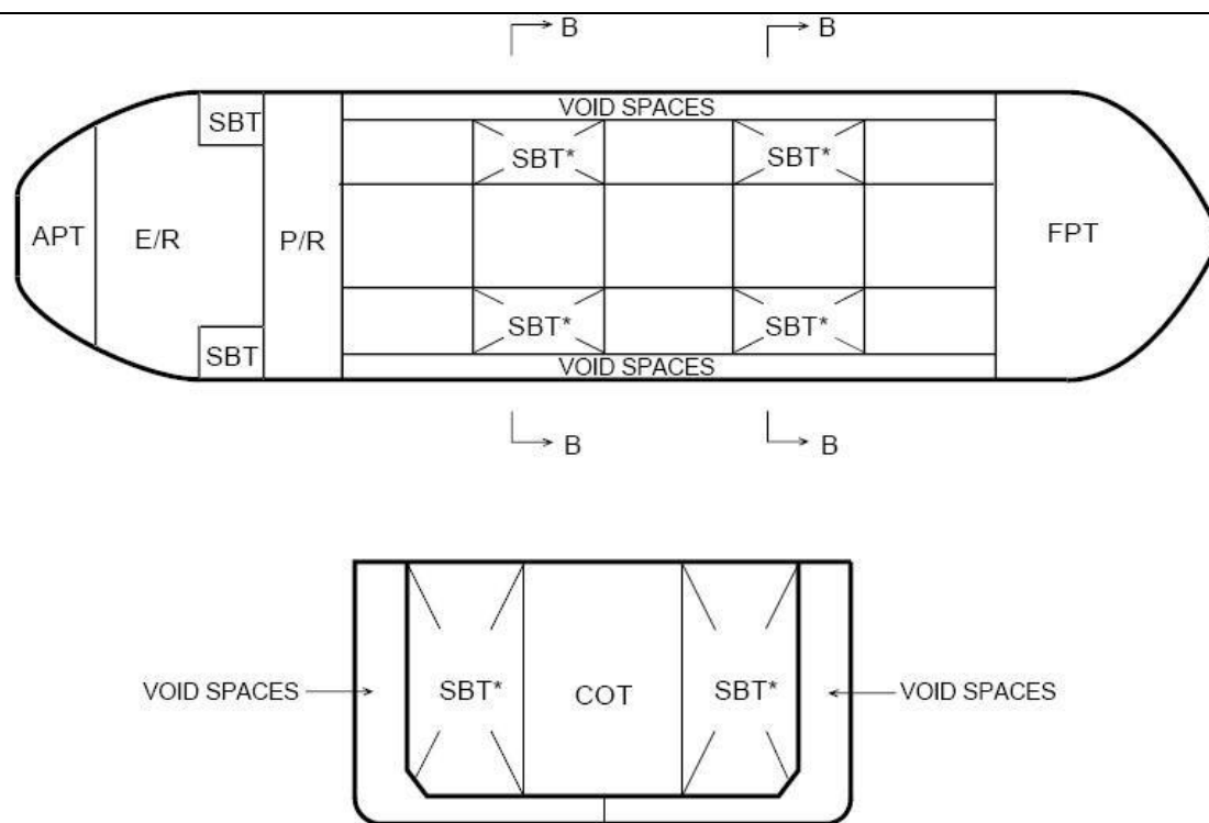
SECTION B-B
