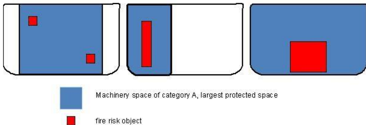
Figure 2 Machinery space not including a casing
