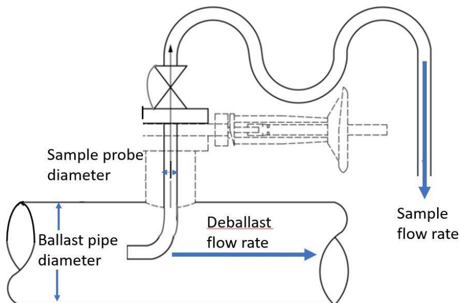
Figure 1 Example of a sample probe in a ballast pipe
