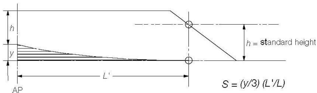
Fig. 3 Sheer credit s for excess height
